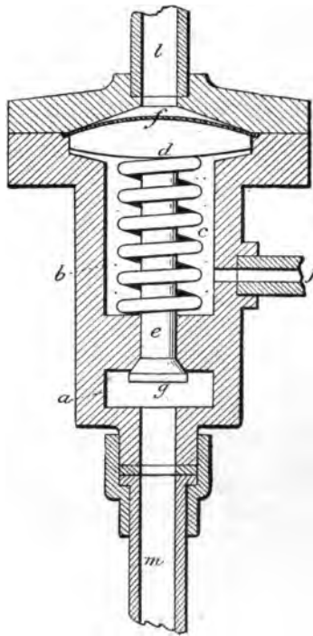
FIG. 359.—Section of the Automatic Boiler Feed Regulator of the White Steam Carriage.
